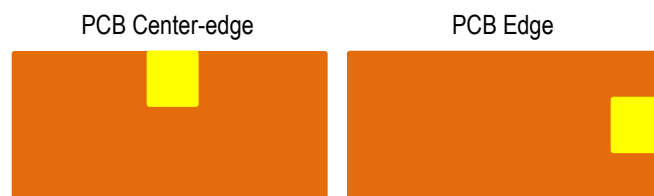
Recommended mounting locations for this antenna
