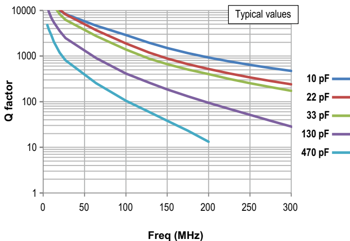
2525 - Q factor
