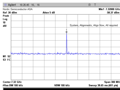
Mid +4dBm 4th harmonic
