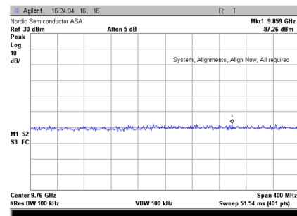
Mid 0dBm 4th harmonic
