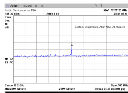
Mid 0dBm 5th harmonic
